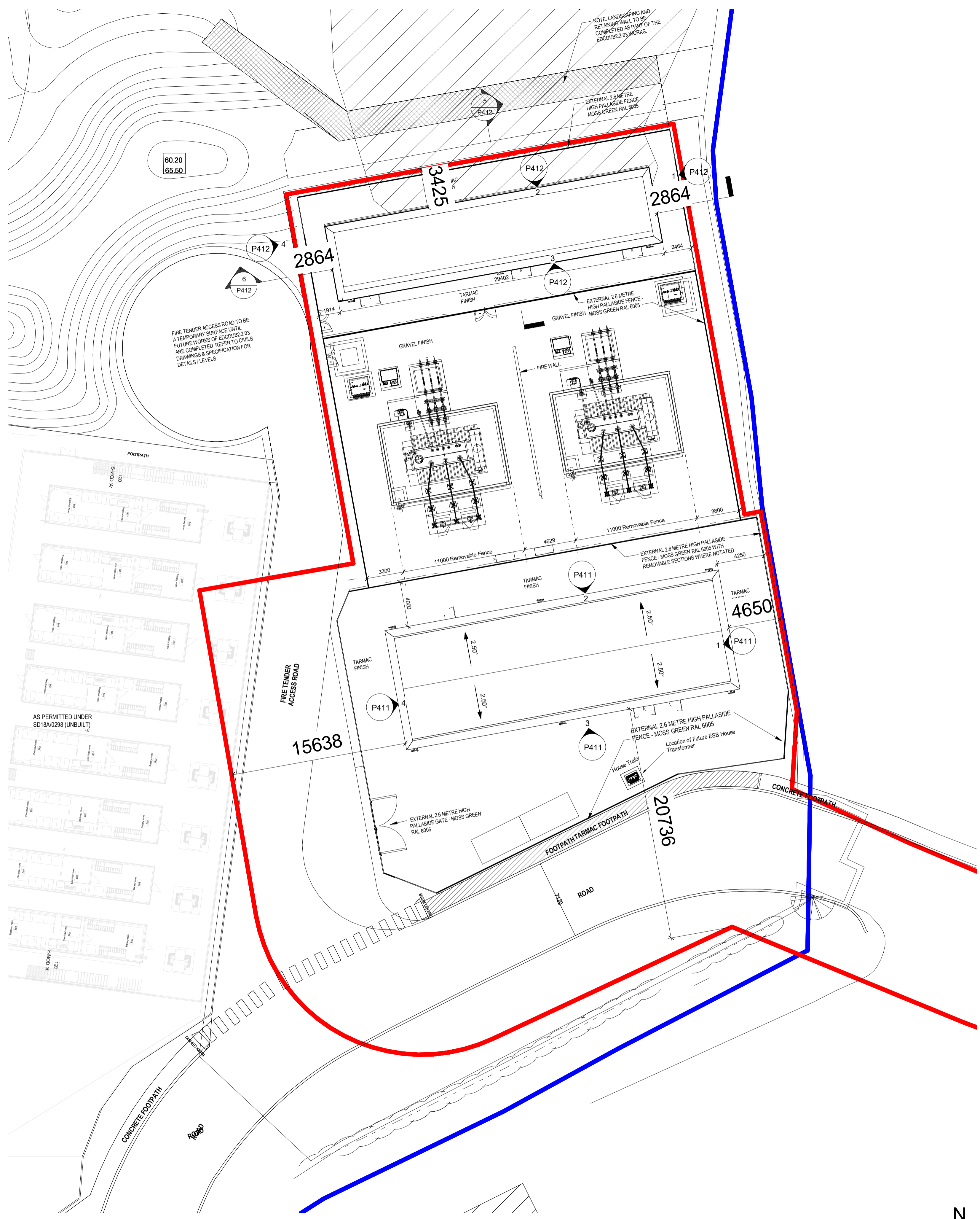
1 PERMITTED SUBSTATION LAYOUT AS GRANTED UNDER SD18A/0298 SCALE: 1 : 200
